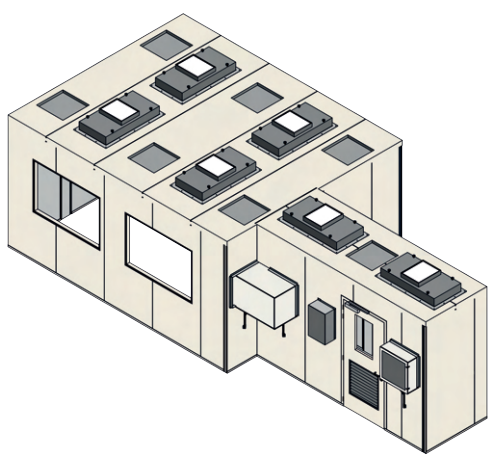
Panelbloc cleanrooms
